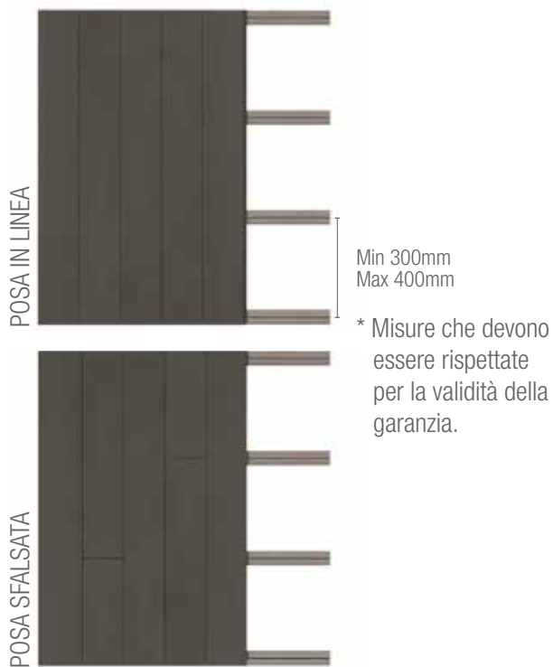
3.3 Posa verticale
